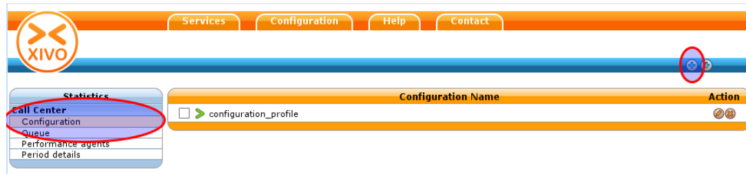
Fig. 1.97: Statistics Configuration
