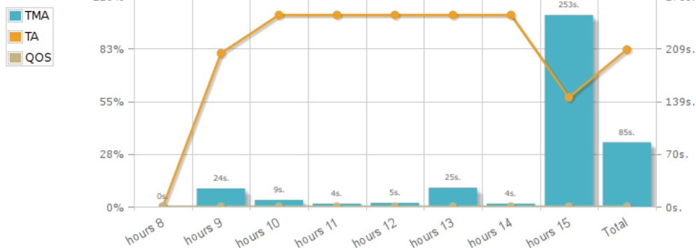
Queues Performance
