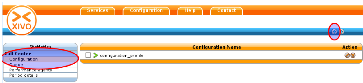
Fig. 1.97: Statistics Configuration
