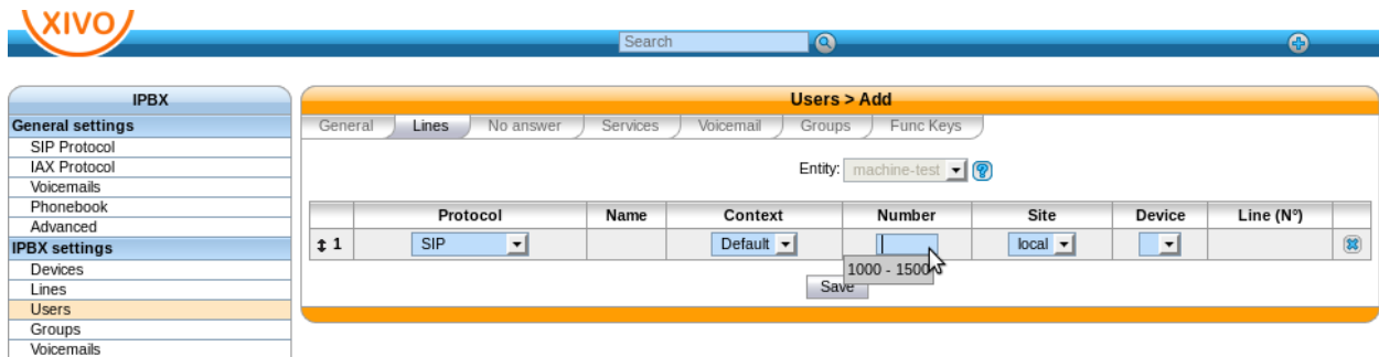
Fig. 1.12: Line information
