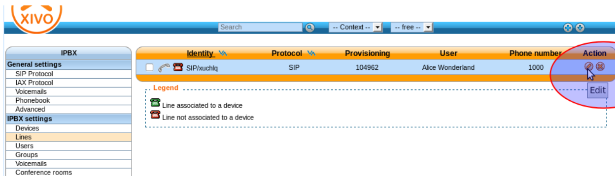
Fig. 1.16: Edit line
